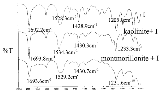
Figure 6. IR spectra of I in clays.
