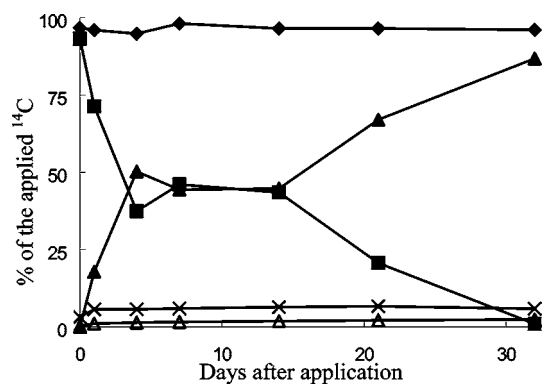
Figure 3. Nitration rate of I on kaolinite. Total ^{14} C ( \blacklozenge ), I ( \square ), XI ( \blacktriangle ), others ( \times ), and bound ^{14} C ( \triangle ).
