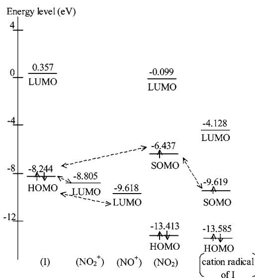
Figure 7. Energy levels of HOMO, SOMO, and LUMO of I and related species estimated by the AM1 MO calculation.
