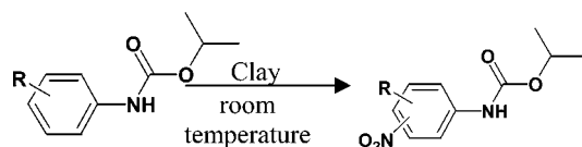
Figure 1. Chemical structure of carbamates and their nitro derivatives in clay-catalyzed nitration.
