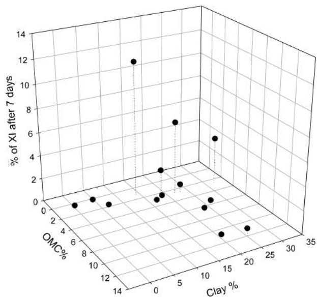
Figure 2. Three-dimensional plot of percent XI vs organic matter content (OMC %) and clay content (clay %).
