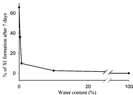
Figure 4. Effect of water content on formation of XI in the kaolinite thin layer.
