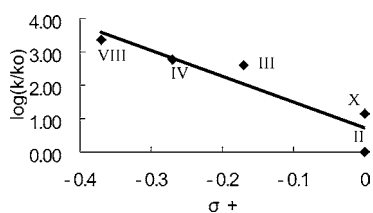
Figure 5. Hammett plot for the nitration of the carbamate analogues.
